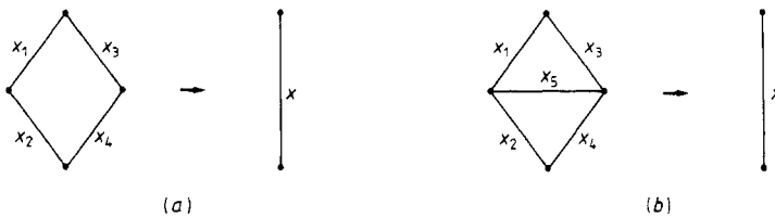
Figure 1. The renormalisation transformations for two hierarchical lattices on which (a) disorder becomes relevant at \alpha_p = 0 , (b) disorder becomes relevant for \alpha_p > -0.0525 .
